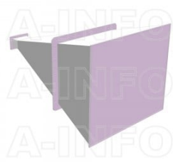
LB-650-20-ASPO Standard Gain Horn Antenna 1.12-1.7GHz 20dB Gain Rectangular Waveguide Interface
