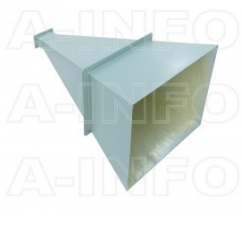
LB-650-20-A Standard Gain Horn Antenna 1.12-1.7GHz 20dB Gain Rectangular Waveguide Interface
