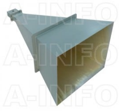
LB-650-20-C-SF Standard Gain Horn Antenna 1.12-1.7GHz 20dB Gain SMA Female
