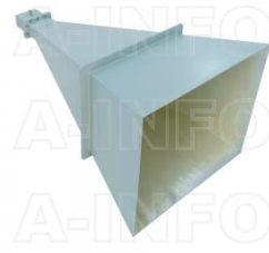
LB-650-20-C-7/16F Standard Gain Horn Antenna 1.12-1.7GHz 20dB Gain 7/16(DIN) Female
